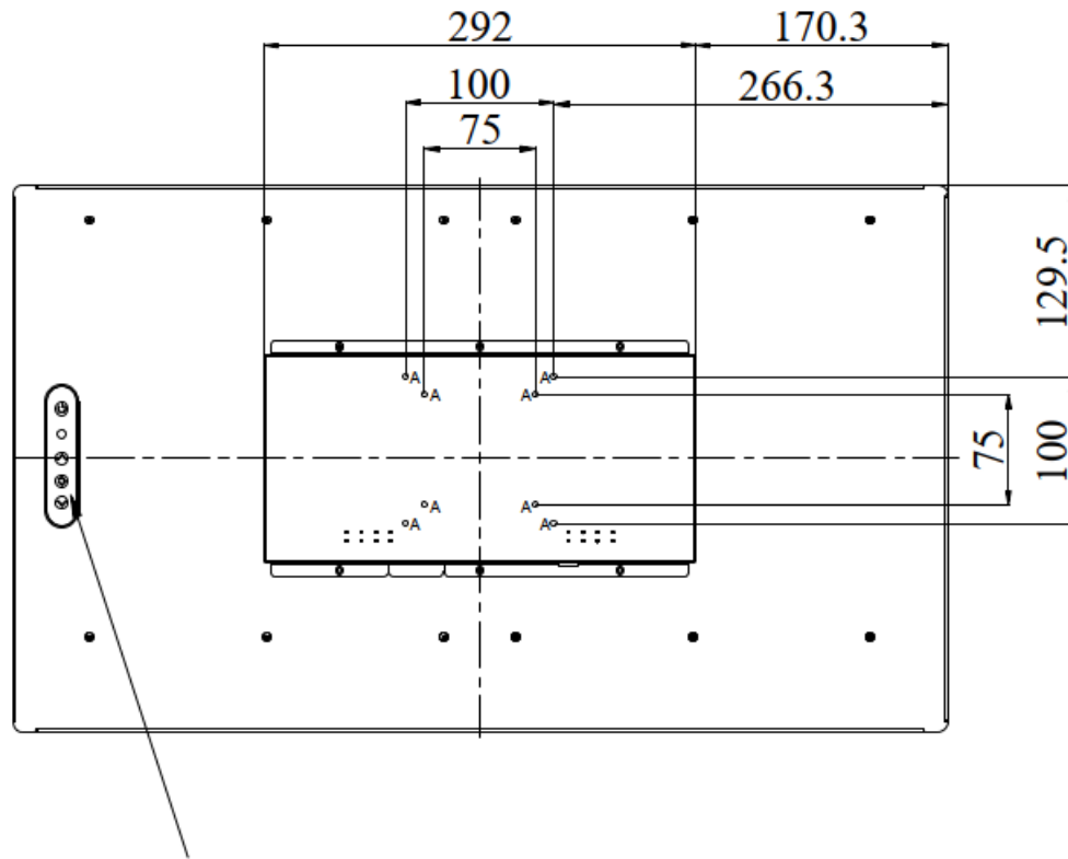
MEMBRANE 4-KEYS
